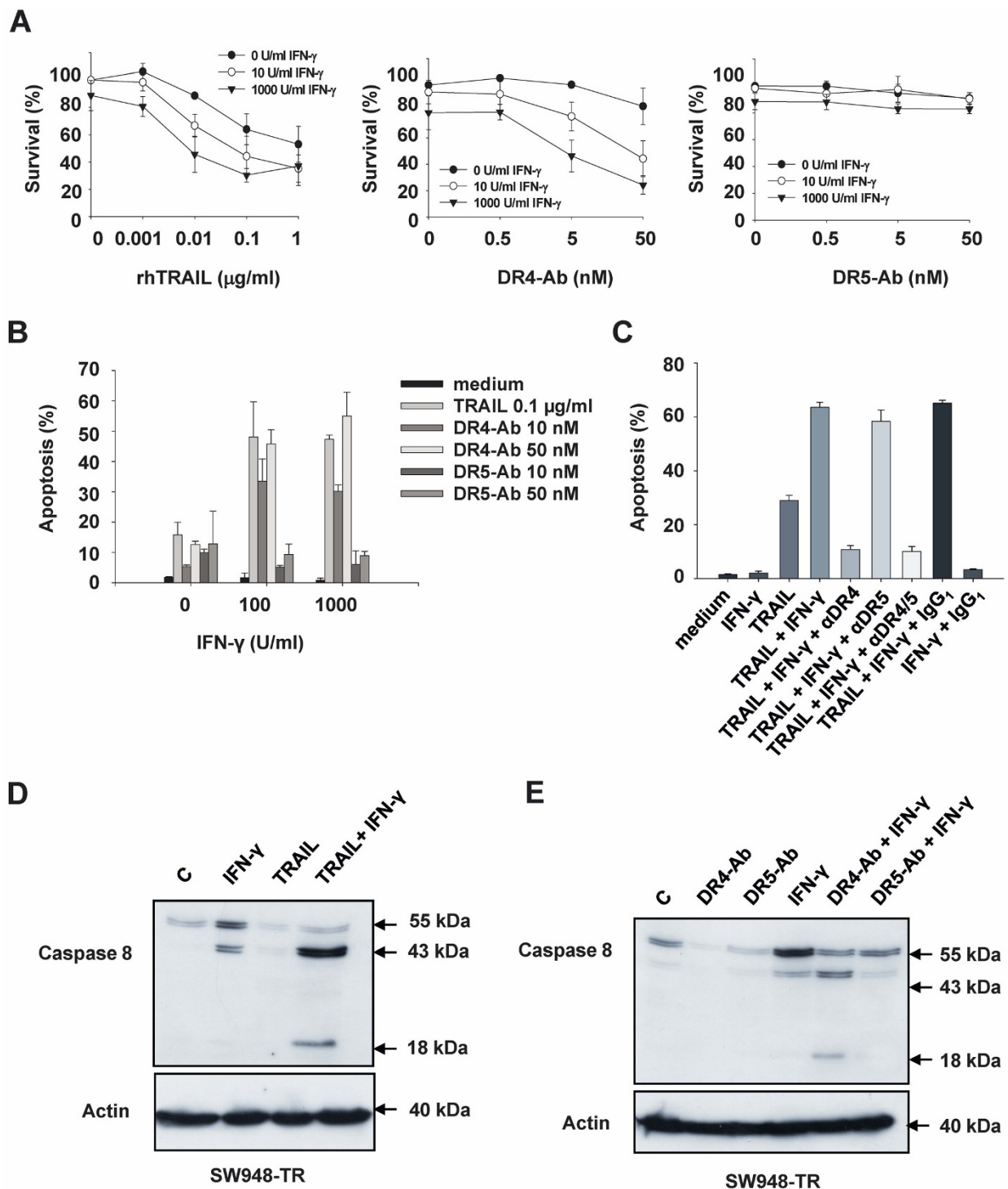
Figure 7 Stimulation of rhTRAIL- and agonistic DR4 antibody-induced but not agonistic DR5 antibody-induced apoptosis by IFN- \gamma . A: Survival (%) of SW948-TR cells after continuous incubation with rhTRAIL, agonistic DR4 or DR5 antibody in combination with different concentrations of IFN- \gamma . B: Apoptosis assay of SW948-TR after 48 h incubation with rhTRAIL, agonistic DR4 or DR5 antibody in combination with various concentrations of IFN- \gamma . C: Apoptosis assay in SW948-TR after 48 h incubation with 1000 U/ml IFN- \gamma . Cells were then incubated with 10 \mu g/ml antagonistic anti-DR4 ( \alpha DR4), anti-DR5 ( \alpha DR5) antibodies, both ( \alpha DR4/5) or IgG1 control for 1 h before 4-5 h rhTRAIL treatment (0.1 \mu g/ml). D: Western blot analysis of caspase 8 activation in SW948-TR cells. The cells were pre-incubated for 48 hours with 1000 U/ml IFN- \gamma , then either left untreated or exposed for 4-5 additional hours with rhTRAIL (0.1 \mu g/ml) before harvest. E: Western blot analysis of caspase 8 activation in SW948-TR cells. The cells were pre-incubated for 48 hours with 1000 U/ml IFN- \gamma , then either left untreated or exposed for 4-5 additional hours with agonistic DR4 antibody (50 nM) or agonistic DR5 antibody (50 nM) before harvest.
