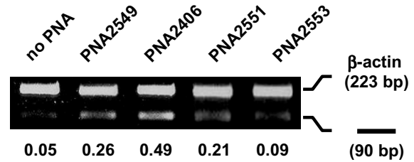
Figure 4 Effect of PNAs on the splicing of intron2. Comparison of PNAs 2549, 2406, 2551 and 2553 in terms of splicing inhibition of intron2 in mdm2 pre-mRNA. JAR cells were transfected with PNAs (2 μM) for 24 h and subjected to RT-PCR analysis using extracted total RNA. RT-PCR was performed with primer sets B and H (see Table 2), for intron2 in mdm2 pre-mRNA (90 bp) and β-actin (223 bp) (as internal control), respectively. RT-PCR results with 27 PCR cycles are shown. The numbers under the figure indicate the relative amount (normalized to β-actin) of the target mdm2 splicing variant.
