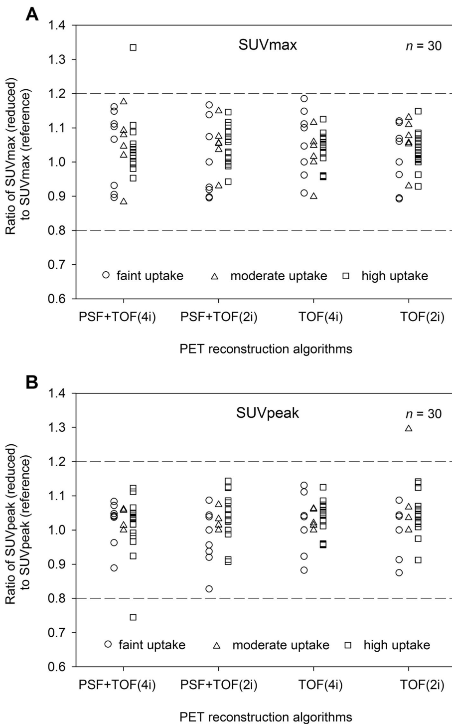
Fig. 2 Dot plots showing the ratio between lesion SUVmax (panel a) and SUVpeak (panel b) between images acquired with reference vs. reduced acquisition protocol. Quantitative assessment was performed separately for lesions with faint (circles, SUVmax≤5), moderate (triangles, 5< SUVmax< 10)), and high uptake (squares, SUVmax ≥ 10). Dashed lines indicate the maximum tolerated deviation of ±20%
