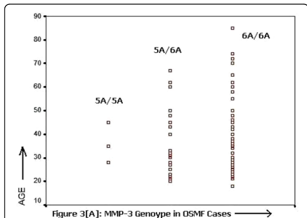
Figure 3[A]: MMP-3 Genotype in OSMF Cases
